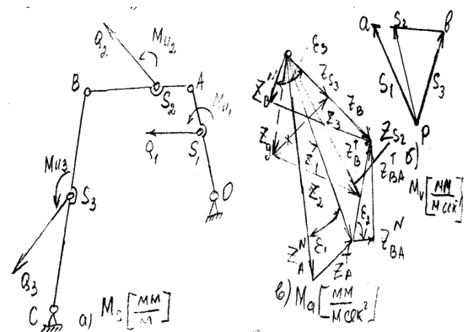
Figure (a-c): Depicting the centers of gravity of the links.
